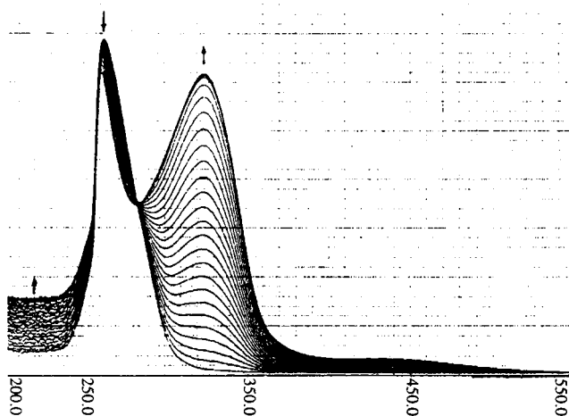
Figure 1. The time-resolved uv spectra of 2a at 50° in dimethyl sulfoxide solution; concentration = 5.04 \times 10^{-5} mol/l; interval: 20 minutes.
